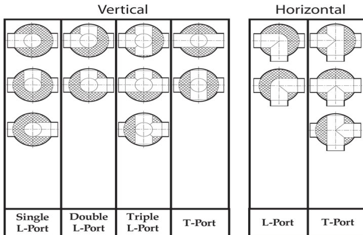
Ball port options viewed from top of valve
