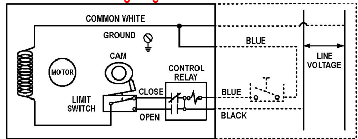
ELECTRO WIRING
