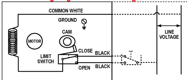
ELECTRO WIRING
